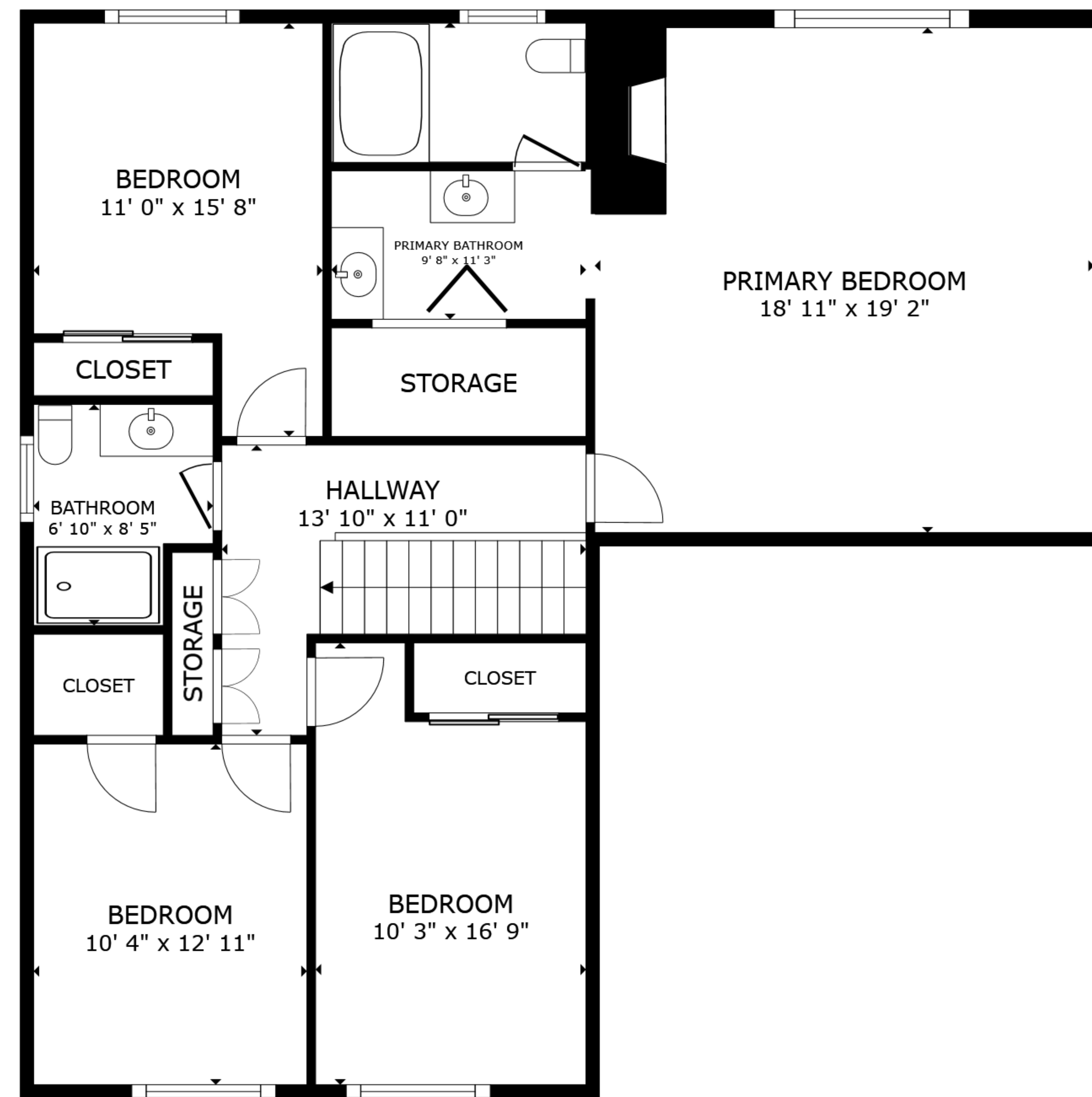
FLOOR 2
